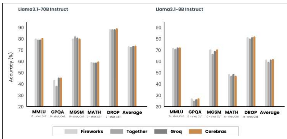
Figure 9-8. An inference service provider might use optimization techniques that can alter a model's behavior, causing different providers to have slight model quality variations. The experiment was conducted by Cerebras (2024).
